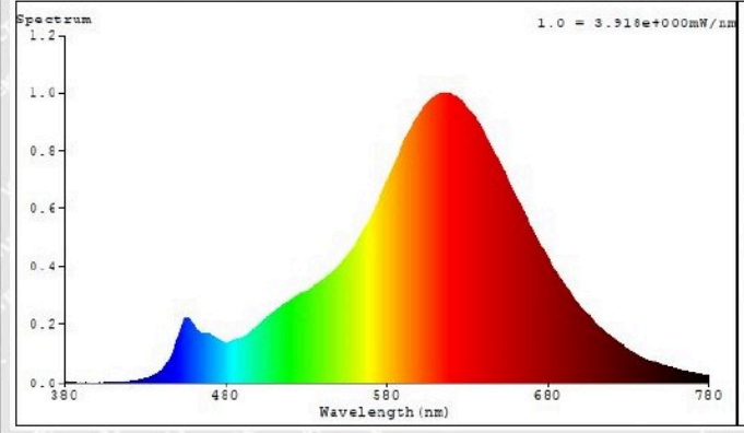
Model: SYSO-2024-S1 (2200K)
